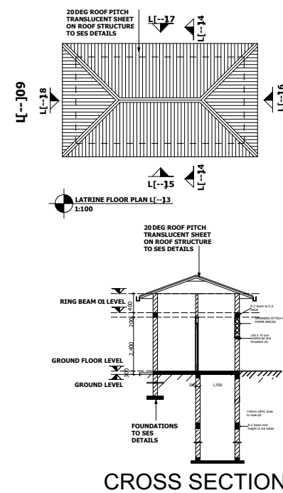
PIT LATRINE FLOOR PLAN
