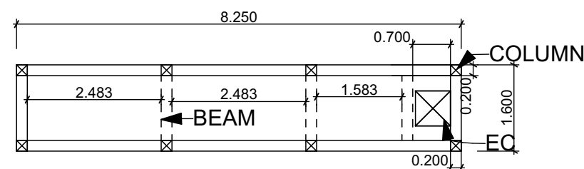
LATRINE FLOOR PLAN PIT LAYOUT
