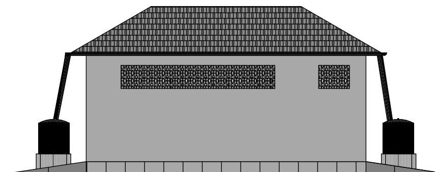
FRONT ELEVATION Elevation 1:100
