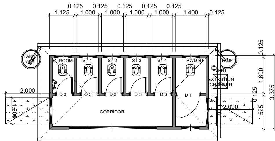
PIT LATRINE FLOOR PLAN
